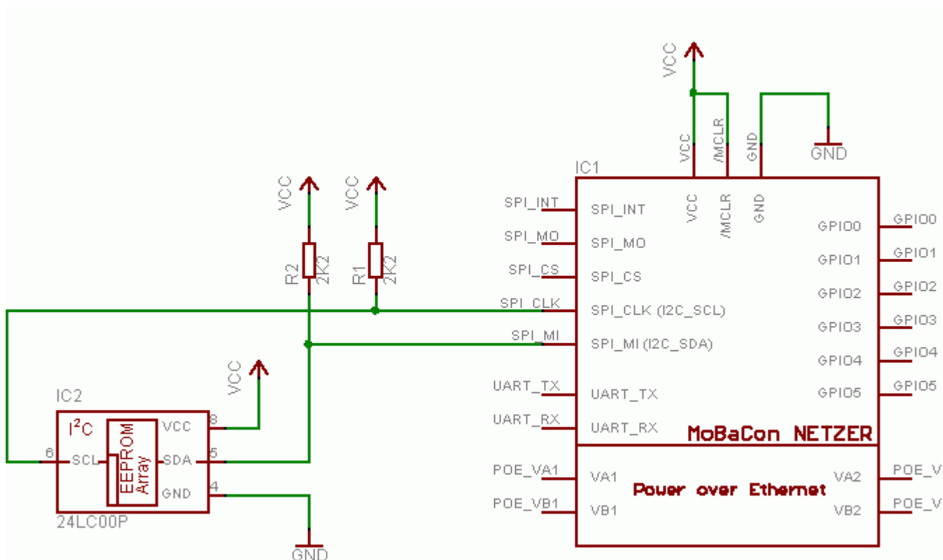
Fig. 1: Connecting a simple EEPROM to Netzer
