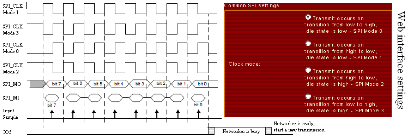
Fig. 2: Waveforms
